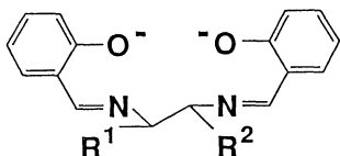
sal-( RR )-chxn
