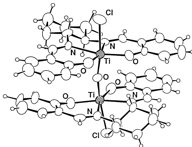
Fig. 1. An ORTEP drawing of [\text{TiCl}(\text{sal-}(\text{RR})\text{-chxn})]_2\text{O} .
